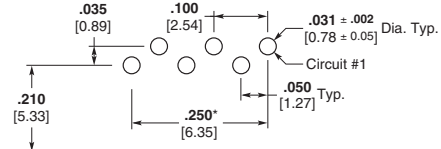
Recommended Mounting Hole Size and Pattern for .062 [1.57] Thick PC Board
